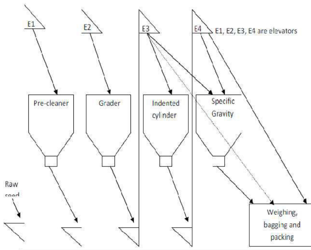
Layout of seed processing machines
